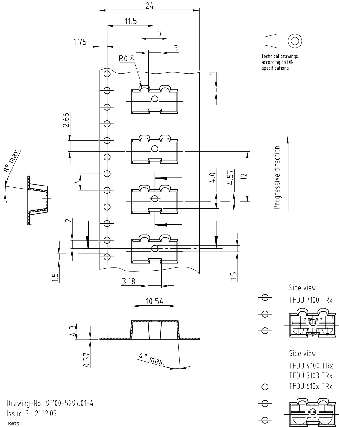
Figure 11. Tape Drawing, TFDU6103 for Side View Mounting, Tolerance ± 0.1 mm
